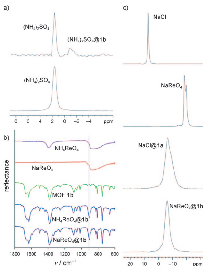
Figure 3. a) ^{15}\text{N} DP-MAS NMR spectra of pure (^{15}\text{NH}_4)_2\text{SO}_4 (bottom) and a sample of 1b prepared by LAG with (^{15}\text{NH}_4)_2\text{SO}_4 (top, w=0.7\% ); b) FTIR-ATR spectra of (top to bottom): \text{NH}_4\text{ReO}_4 , \text{NaReO}_4 , 1b with DMF guest, 1b obtained by ILAG with \text{NH}_4\text{ReO}_4 , and 1b obtained by ILAG with \text{NaReO}_4 ; the vertical line marks the 910\text{ cm}^{-1} band; c) ^{23}\text{Na} DP-MAS NMR spectra (top to bottom) of: \text{NaCl} , \text{NaReO}_4 , 1a obtained by ILAG with \text{NaCl} , 1b obtained by ILAG with \text{NaReO}_4 .
